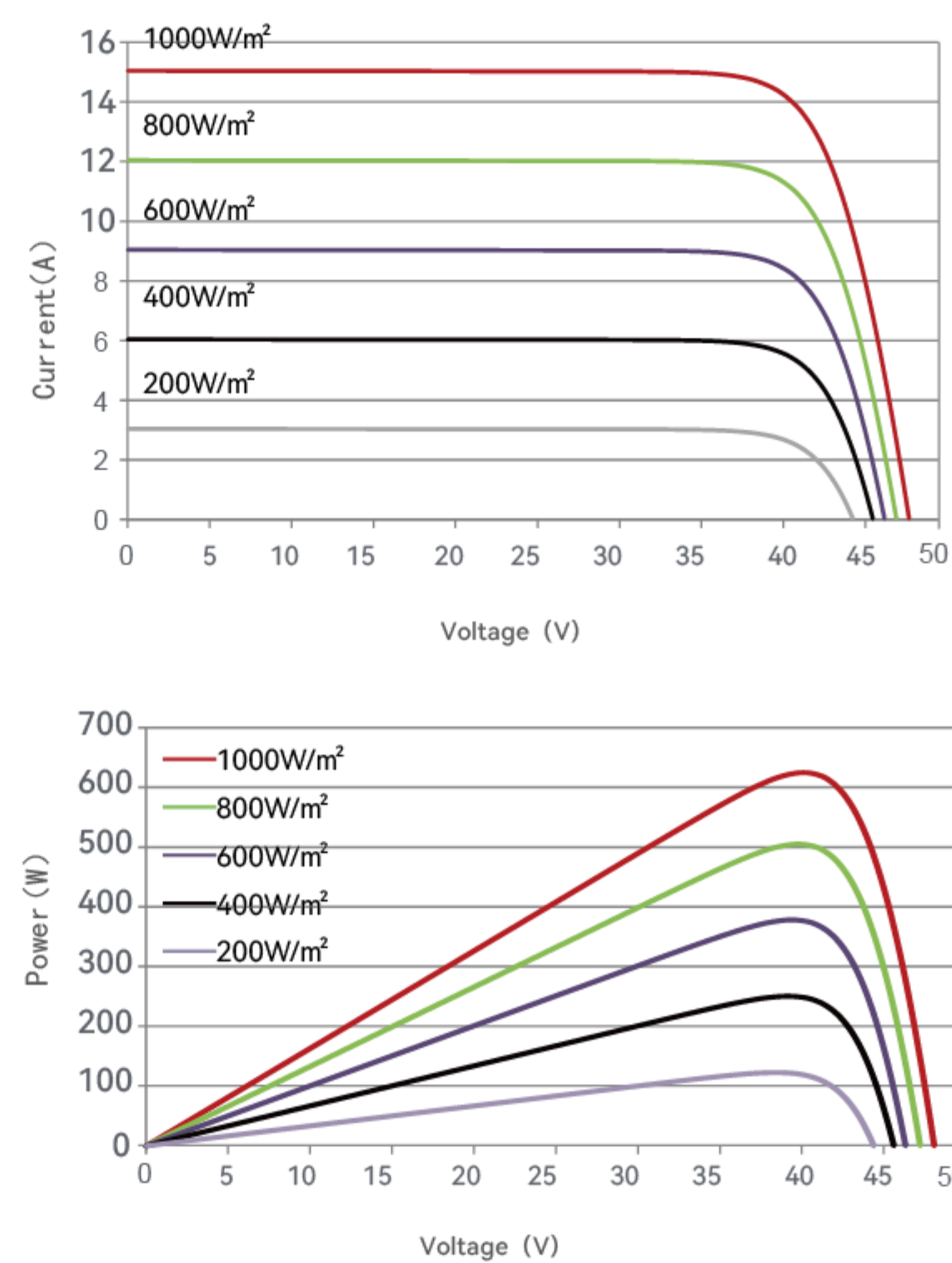
I-V curve
