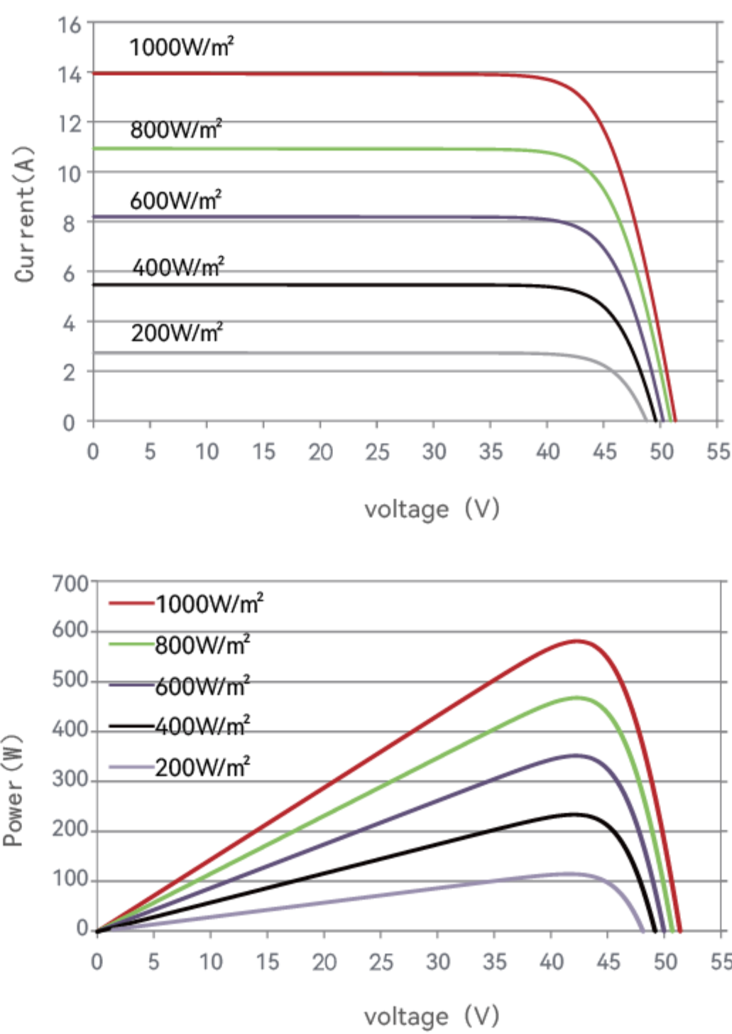
I-V curve
